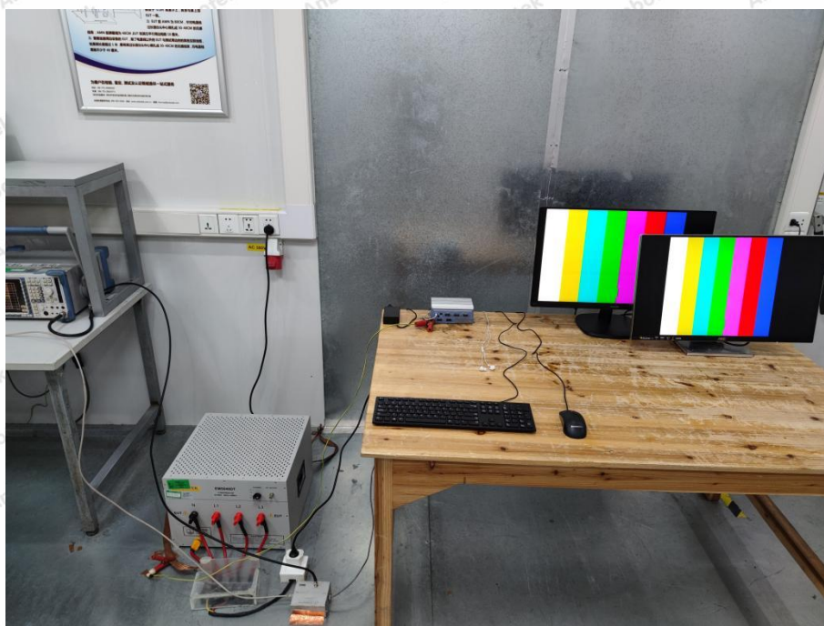
Photo of Asymmetric Mode Conducted Emission at Telecom Port
