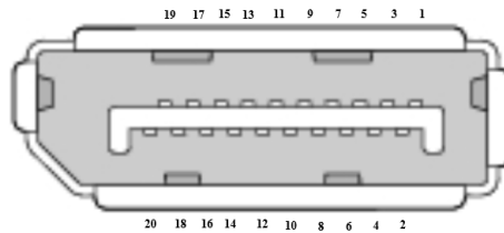
Picture 2.8: DP
