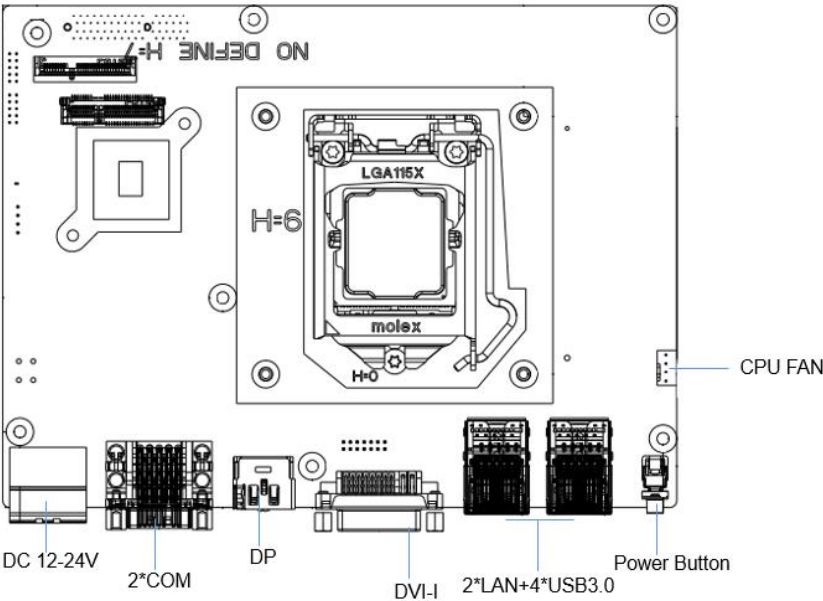
Picture 1.1: STX-I952 Front
