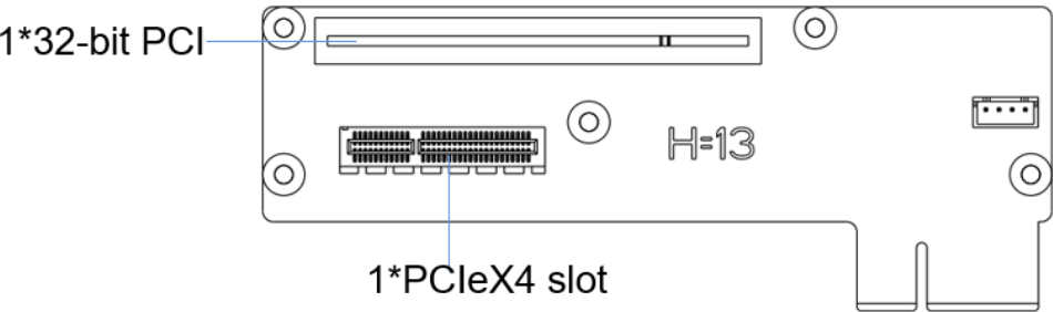
Picture 1.3: ECX-257
