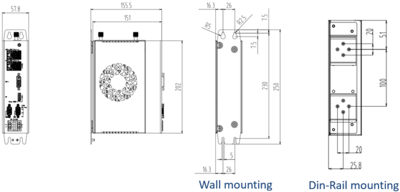
Picture 1.6 KGEC-6300-S001 Dimension
