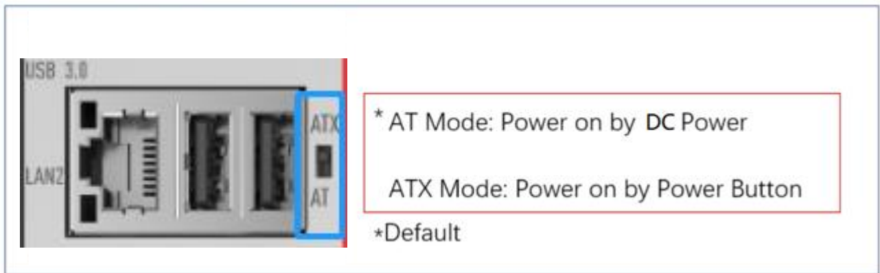
Picture 2.2: AT/ATX
