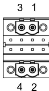
Picture 2.10: DC-IN
