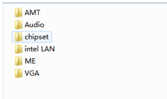
Figure 5.1 win7 drivers
