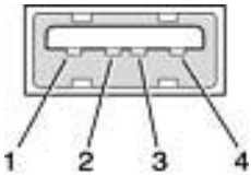
Picture 2.7: USB2.0
