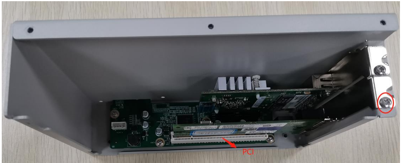
Picture 2.21: PCI installation (2)
