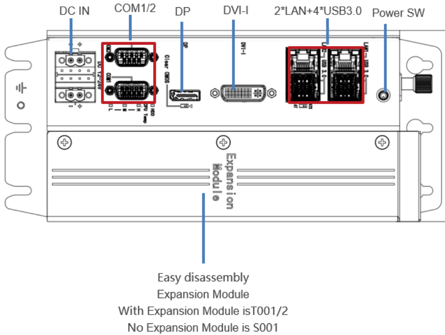
Picture 1.4: KGEC-6300-T002 Front Panel
