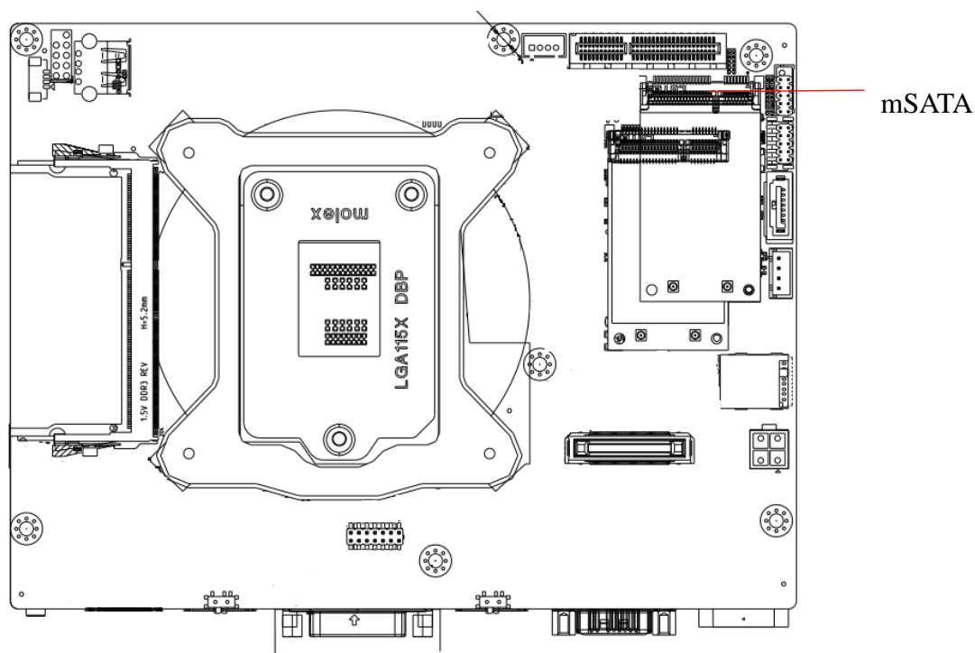
Picture 2.13: mSATA
