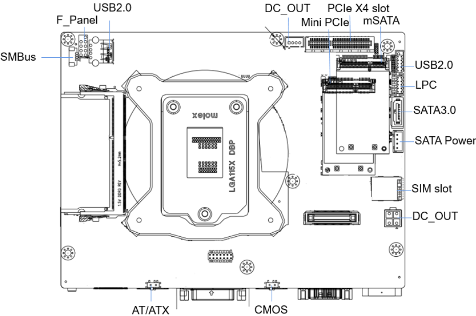
Picture 1.2: STX-I952 Rear
