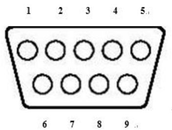
Figure 2.19 COM1/2 Connector
