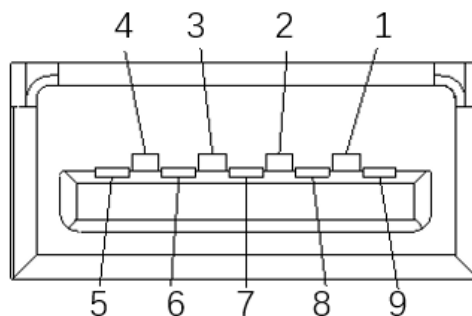
Figure 2.16: USB3.0 Connector
