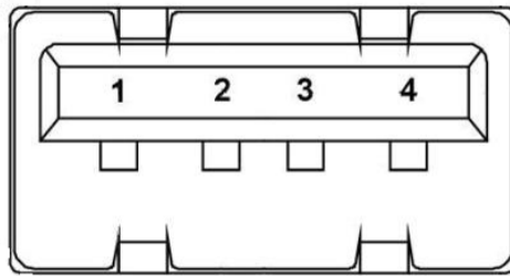
Figure 2.15 USB2.0 connector
