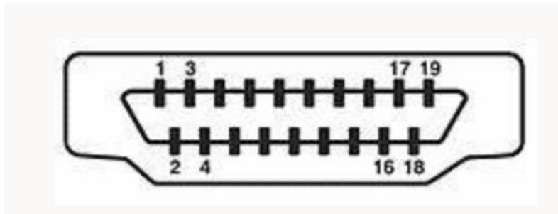
Figure 2.17 HDMI Connector
