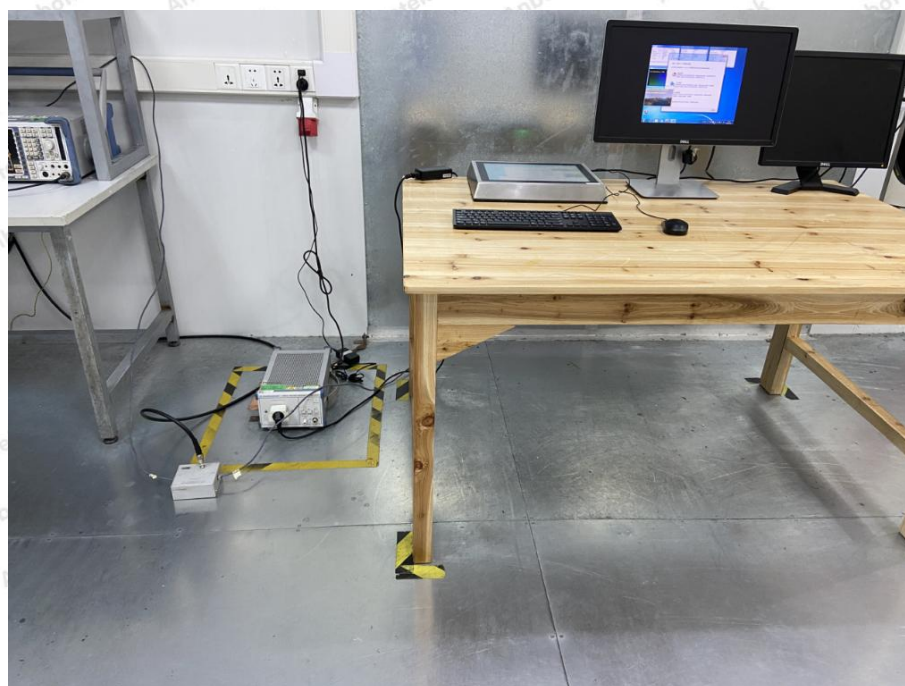
Photo of Asymmetric Mode Conducted Emissions Test
