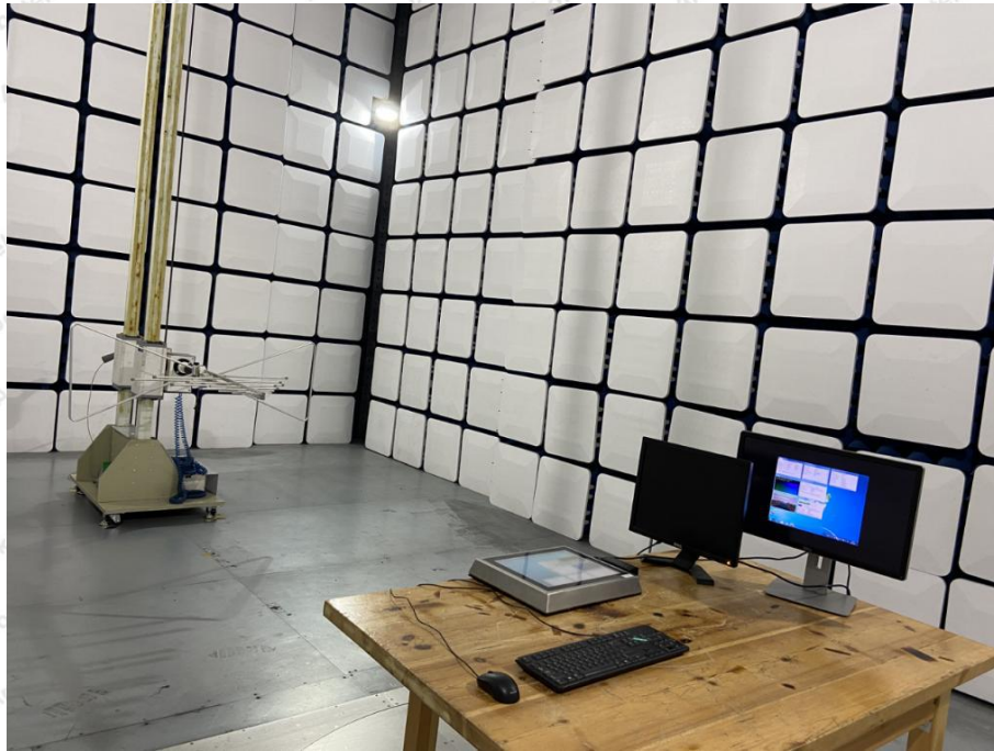
Photo of Radiated Emission Test (30-1000MHz)
