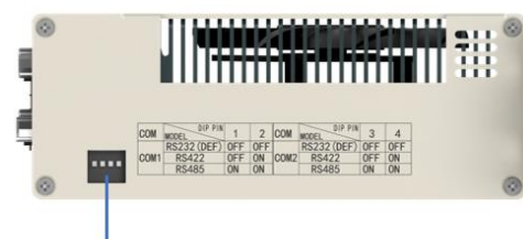
COM selector switch
